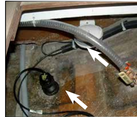
LOG DEPTH SOUNDER SENSOR + AUTOMATIC PILOT COMPASS
